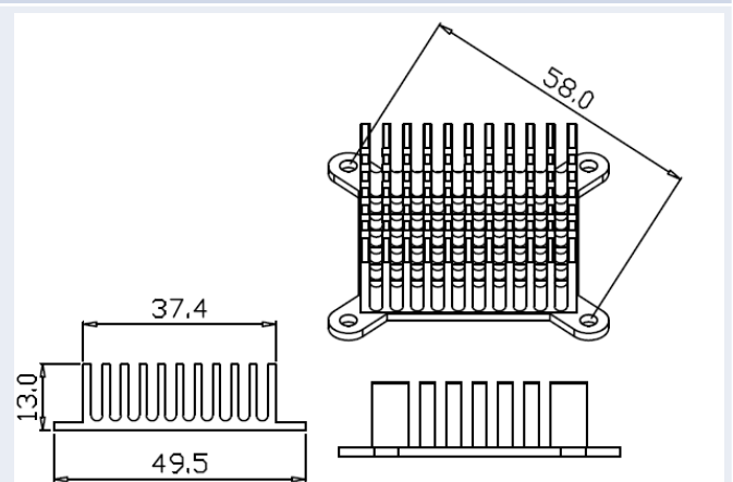
Series Number: RG-CM496X2 Dimension(mm): 49.5x13.0xFree
