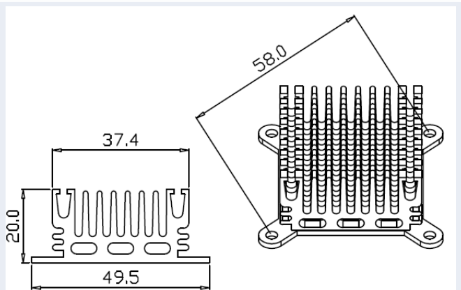
Series Number: RG-CM493X2 Dimension(mm): 49.5x20.0xFree
