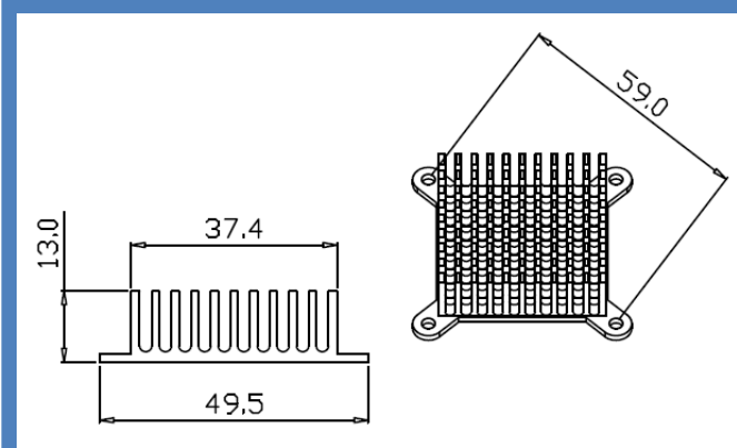
Series Number: RG-CM491X1 Dimension(mm): 49.5x13.0xFree
