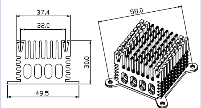
Series Number: RG-CM391X2 Dimension(mm): 49.5x30.0xFree
