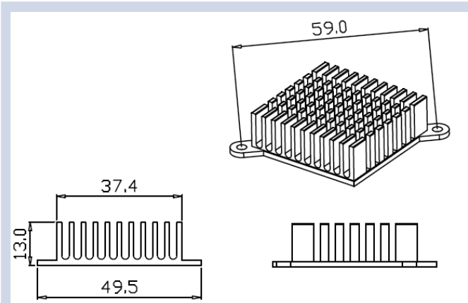
Series Number: RG-CM496A Dimension(mm): 49.5x13.0xFree
