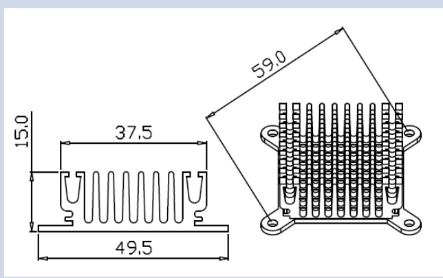
Series Number: RG-CM492X1 Dimension(mm): 49.5x15.0xFree
