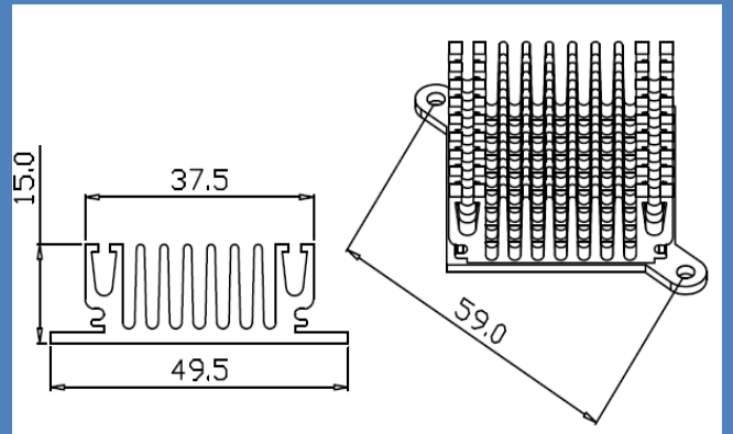
Series Number: RG-CM492B Dimension(mm): 49.5x15.0xFree
