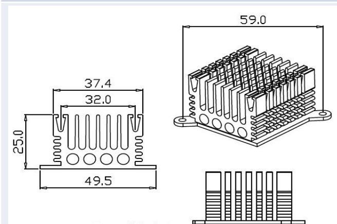
Series Number: RG-CM484A Dimension(mm): 49.5x25.0xFree
