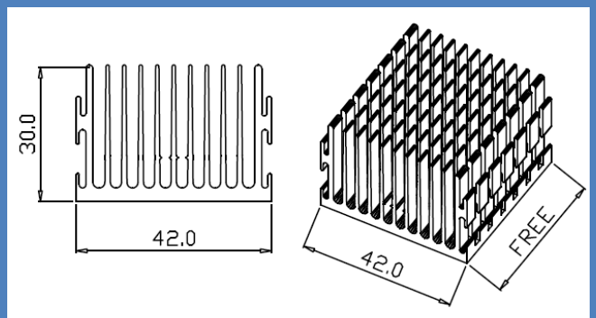
Series Number: RG-CM433 Dimension(mm): 42.0x30.0xFree
