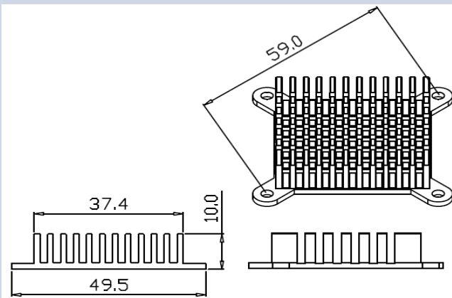
Series Number: RG-CM495X1 Dimension(mm): 49.5x10.0xFree
