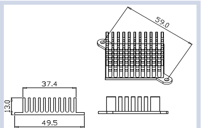
Series Number: RG-CM496B Dimension(mm): 49.5x13.0xFree
