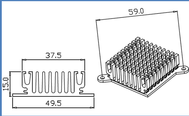
Series Number: RG-CM492A Dimension(mm): 49.5x15.0xFree
