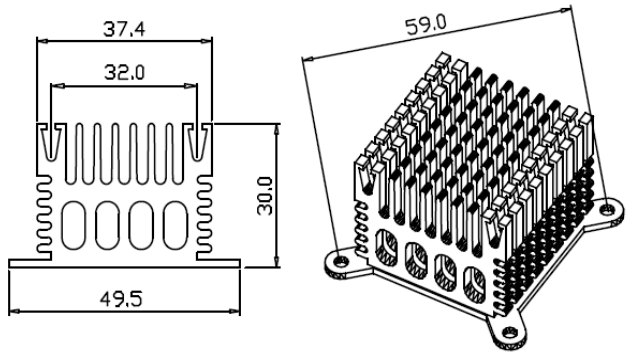
Series Number: RG-CM391X1 Dimension(mm): 49.5x30.0xFree
