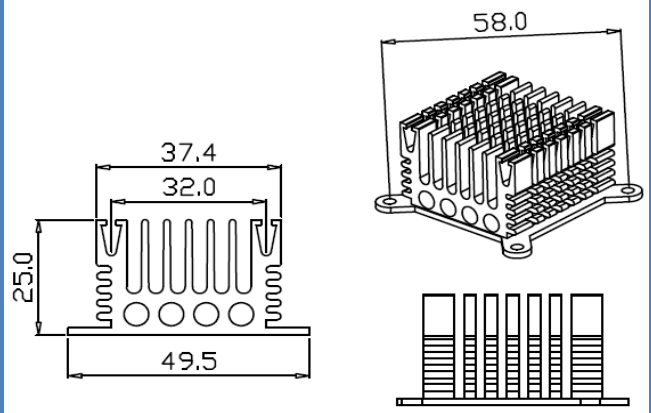
Series Number: RG-CM484X2 Dimension(mm): 49.5x25.0xFree
