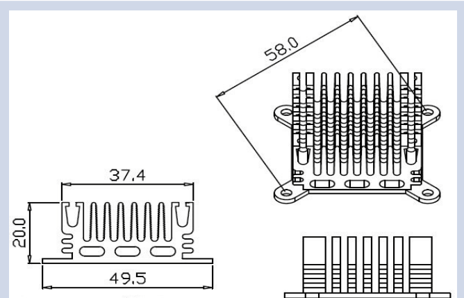
Series Number: RG-CM498X2 Dimension(mm): 49.5x20.0xFree
