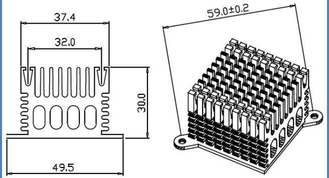
Series Number: RG-CM391B Dimension(mm): 49.5x30.0xFree
