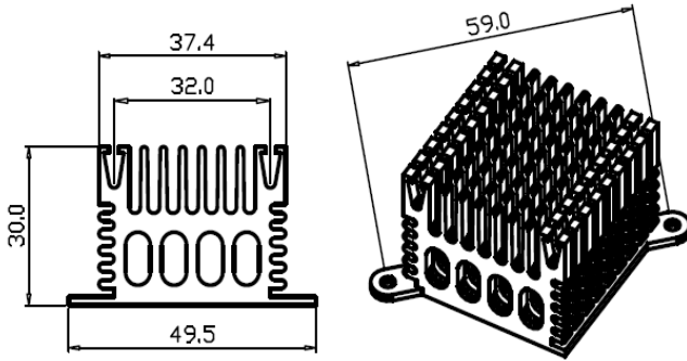
Series Number: RG-CM391A Dimension(mm): 49.5x30.0xFree
