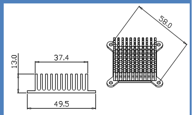
Series Number: RG-CM491X2 Dimension(mm): 49.5x13.0xFree
