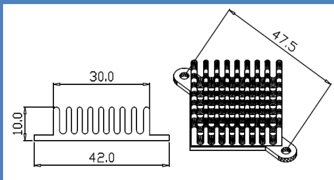
Series Number: RG-CM439B Dimension(mm): 42.0x10.0xFree
