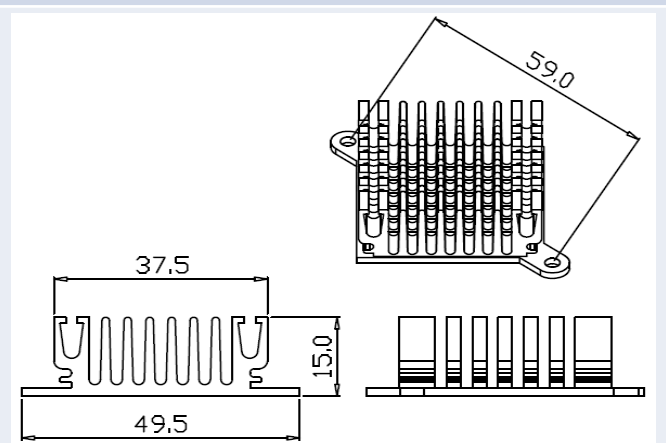
Series Number: RG-CM497B Dimension(mm): 49.5x15.0xFree
