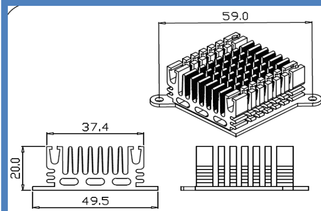
Series Number: RG-CM498A Dimension(mm): 49.5x20.0xFree
