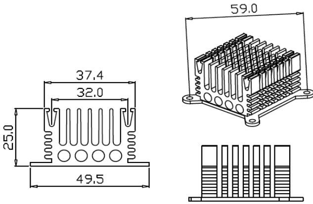
Series Number: RG-CM484X1 Dimension(mm): 49.5x25.0xFree
