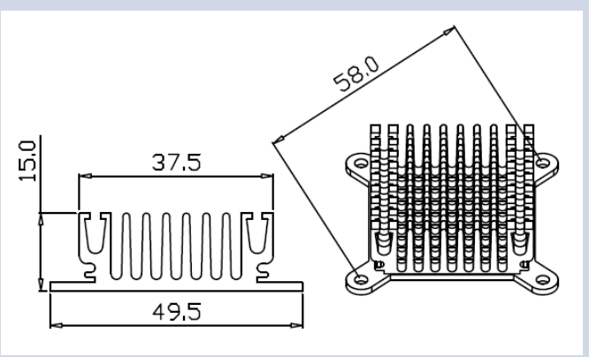
Series Number: RG-CM492x2 Dimension(mm): 49.5x15.0xFree
