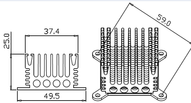
Series Number: RG-CM494A Dimension(mm): 49.5x25.0xFree
