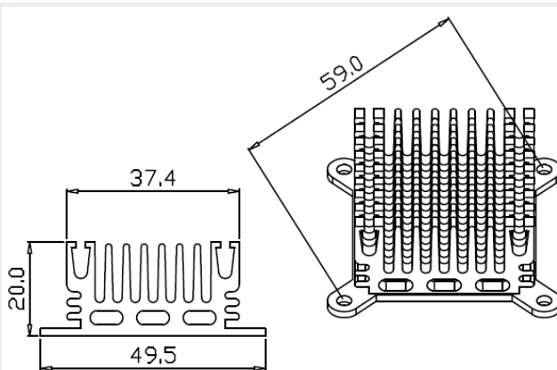
Series Number: RG-CM493X1 Dimension(mm): 49.5x20.0xFree
