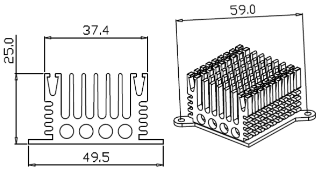
Series Number: RG-CM494A Dimension(mm): 49.5x25.0xFree
