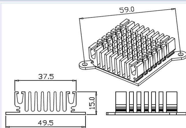
Series Number: RG-CM497A Dimension(mm): 49.5x15.0xFree
