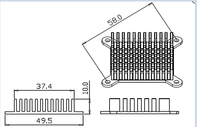
Series Number: RG-CM495X2 Dimension(mm): 49.5x10.0xFree
