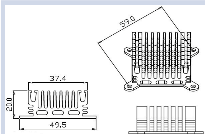
Series Number: RG-CM498X1 Dimension(mm): 49.5x20.0xFree
