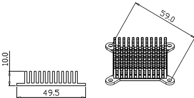
Series Number: RG-CM490A Dimension(mm): 49.5x10.0xFree
