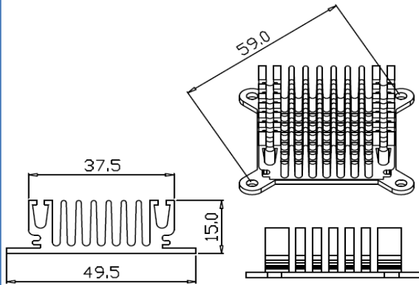
Series Number: RG-CM497X1 Dimension(mm): 49.5x15.0xFree
