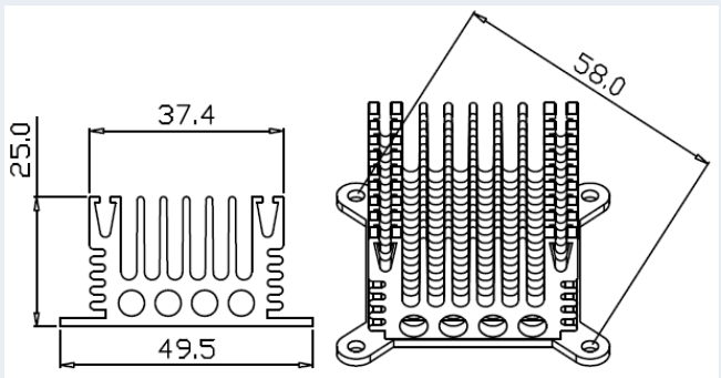
Series Number: RG-CM494B Dimension(mm): 49.5x25.0xFree
