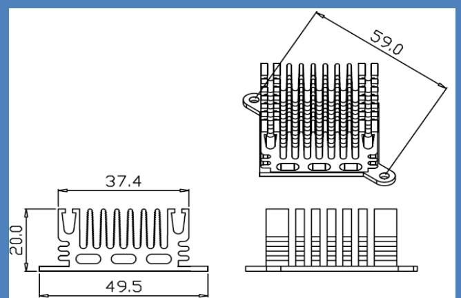
Series Number: RG-CM498B Dimension(mm): 49.5x20.0xFree
