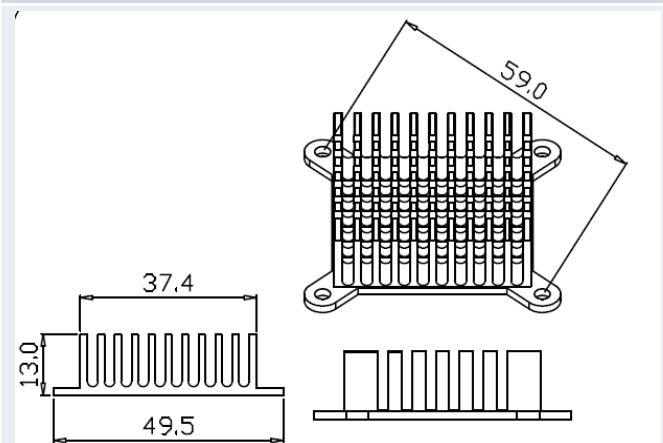
Series Number: RG-CM496X1 Dimension(mm): 49.5x13.0xFree
