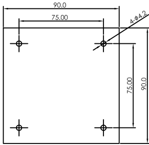
PCB LAYOUT
